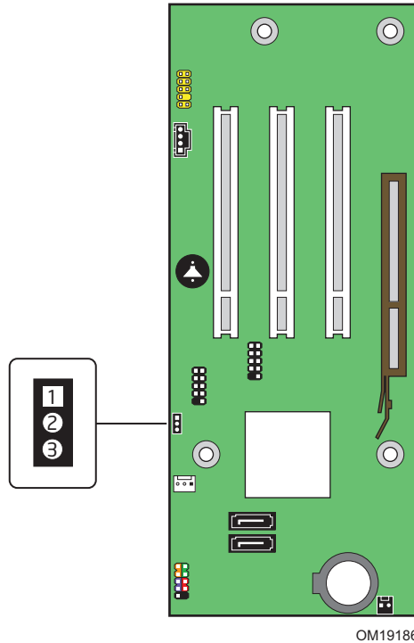
Figure 24. Location of the BIOS Configuration Jumper Block
